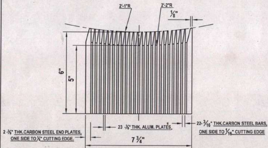
ASSEMBLY DETAIL FROM SIDE VIEW
